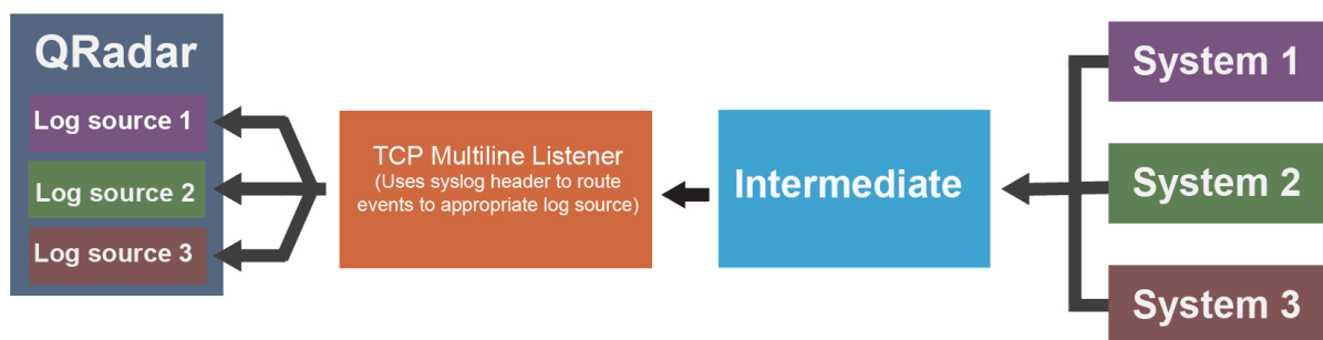
Figure 4. Separate QRadar log sources collect events sent from multiple systems and forwarded via an intermediate system to a TCP Multiline Listener, by using the syslog header.
